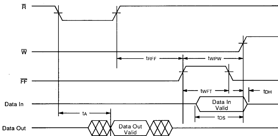
Figure 11. Write Data Flow-Through Mode
