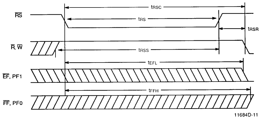
Figure 7. Reset Timing Diagram
