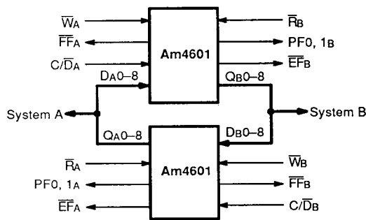
Figure 3. Bidirectional FIFO Mode
