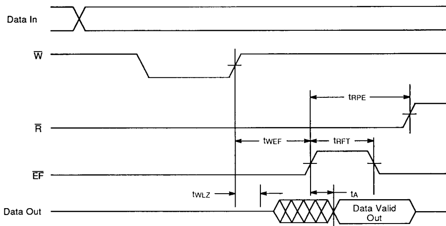
Figure 10. Read Data Flow-Through Mode
