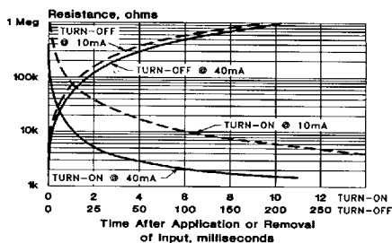
Response Time VTL5C3/2
