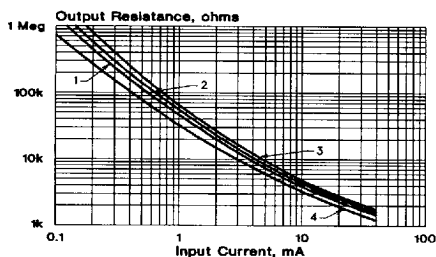
Output Resistance vs Input Current VTL5C3/2
