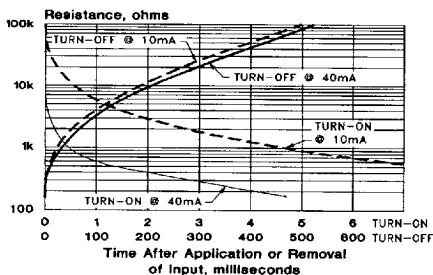
Response Time VTL5C4/2
