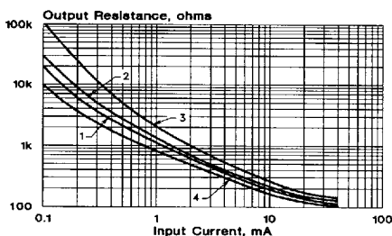
Output Resistance vs Input Current VTL5C4/2
