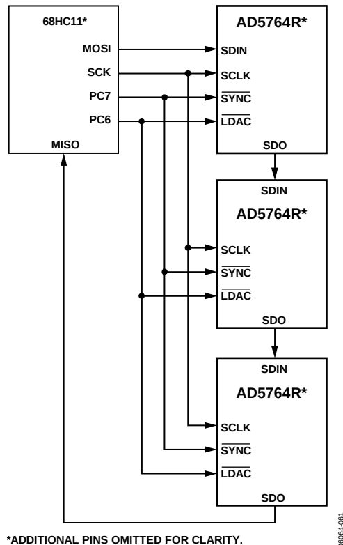
Figure 40. Daisy-Chaining the AD5764R
