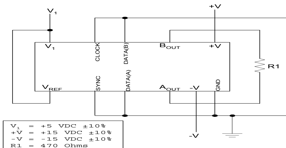
Figure 7: Burn-in Schematic
