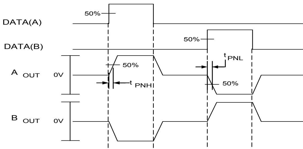
Figure 6: Propagation Delay
