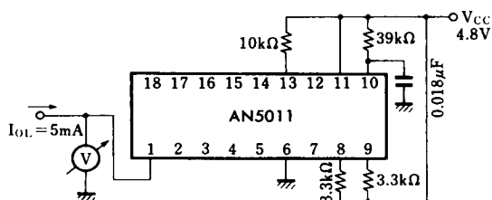
Test Circuit 1 ( V_{OL(K)} )
