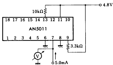
Test Circuit 5 ( I_{IL(CHD)} )
