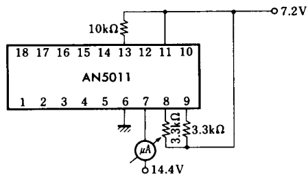
Test Circuit 6 ( I_{IH(CHD)} )
