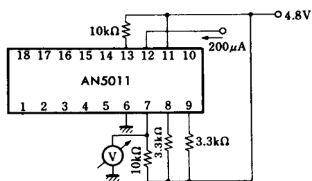
Test Circuit 12 ( I_{IH(SK)} )
