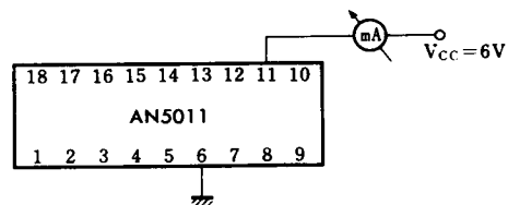
Test Circuit 16 ( I_{tot} )
