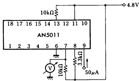
Test Circuit 8 ( I_{IH(CHU)} )
