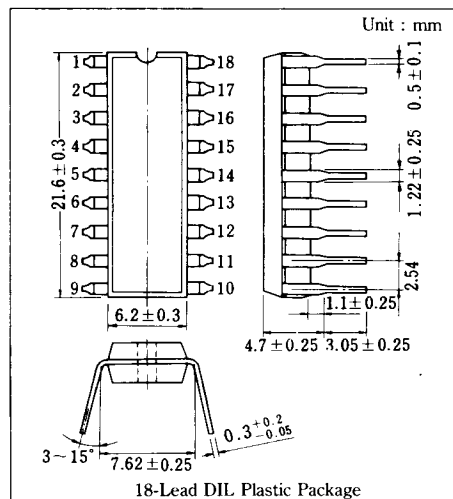
18-Lead DIL Plastic Package
