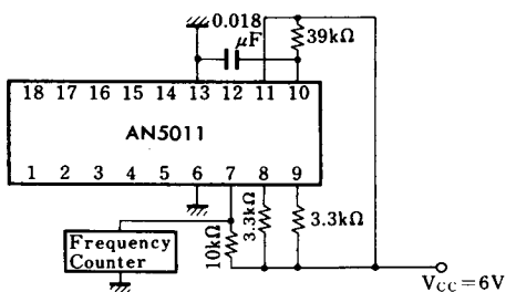
Test Circuit 15 ( f_{OSC} )
