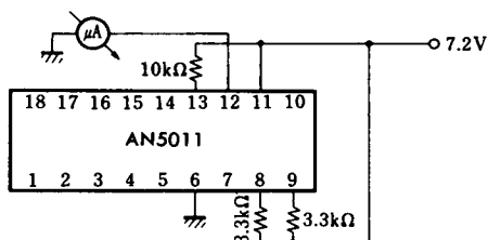
Test Circuit 9 ( I_{IL(KI)} )
