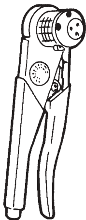
8365 with locator 8365-02
