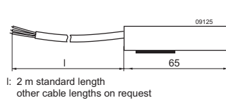
Battery temperature sensor
