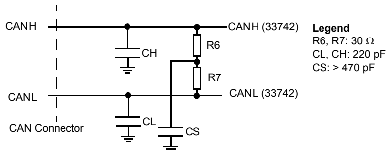
Figure 37. CAN Bus Split Termination
