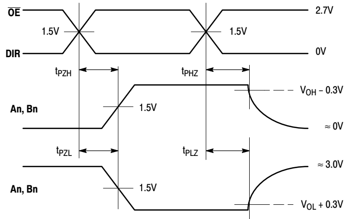
WAVEFORM 2 – OE/DIR to An/Bn OUTPUT ENABLE AND DISABLE TIMES t_R = t_F = 2.5ns , 10% to 90%; f = 1MHz ; t_W = 500ns
