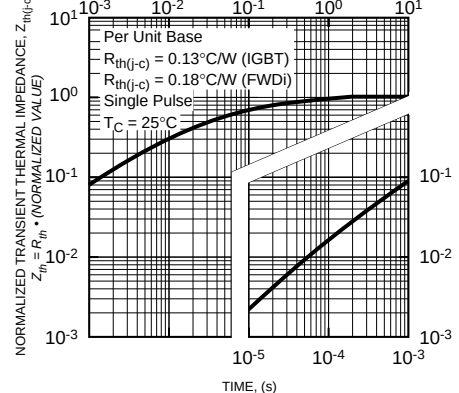
TRANSIENT THERMAL IMPEDANCE CHARACTERISTICS (IGBT & FWD)
