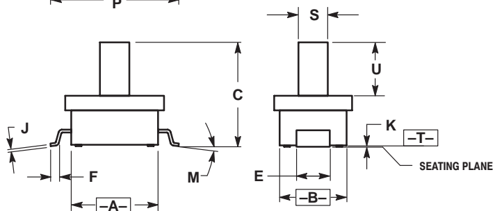
CASE 1320A-02 MPAK, STYLE 2
