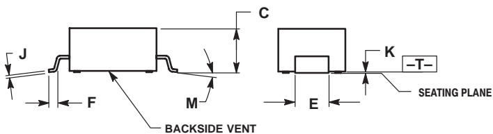
CASE 1320A-02 MPAK, STYLE 1
