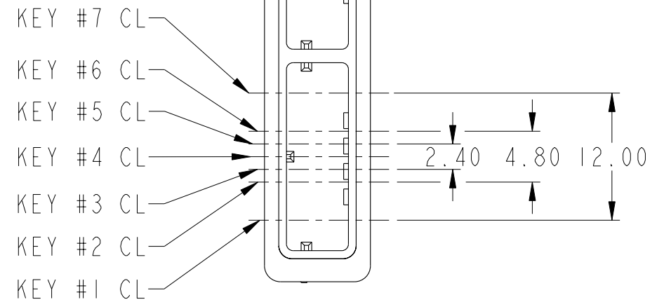
RAIL KEY DIMENSION
