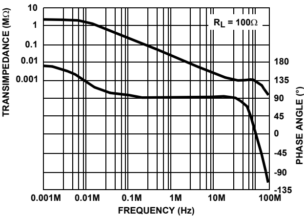
FIGURE 56. TRANSIMPEDANCE vs FREQUENCY
