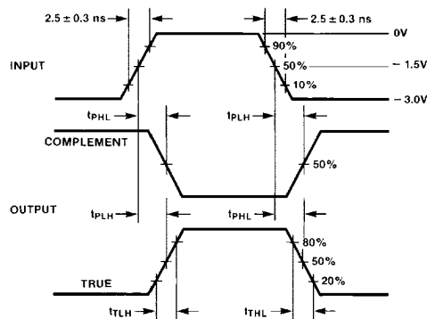
FIGURE 1. Propagation Delay, Cut-Off and Transition Times
