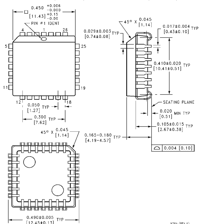
28-Lead Plastic Lead Chip Carrier (PLCC), JEDEC MO-047, 0.450 Square Package Number V28A
