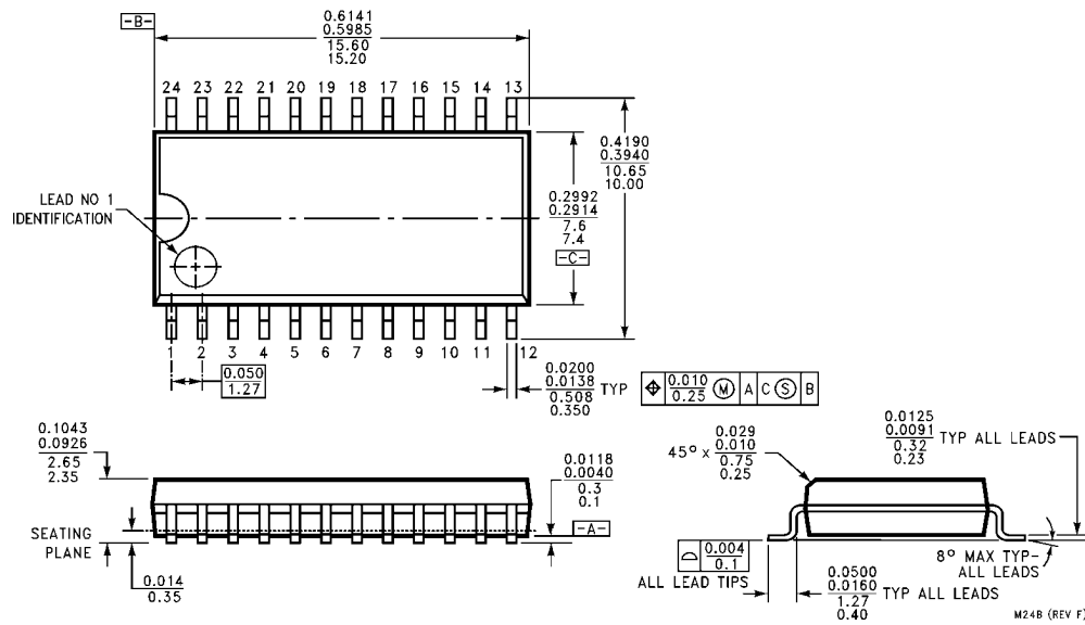
28-Lead Small Outline Integrated Circuit (SOIC), JEDEC MS-013, 0.300 Wide Package Number M24B
