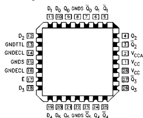
Pin Assignments for 28-Pin PLCC
