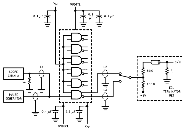
FIGURE 2. AC Test Circuit
