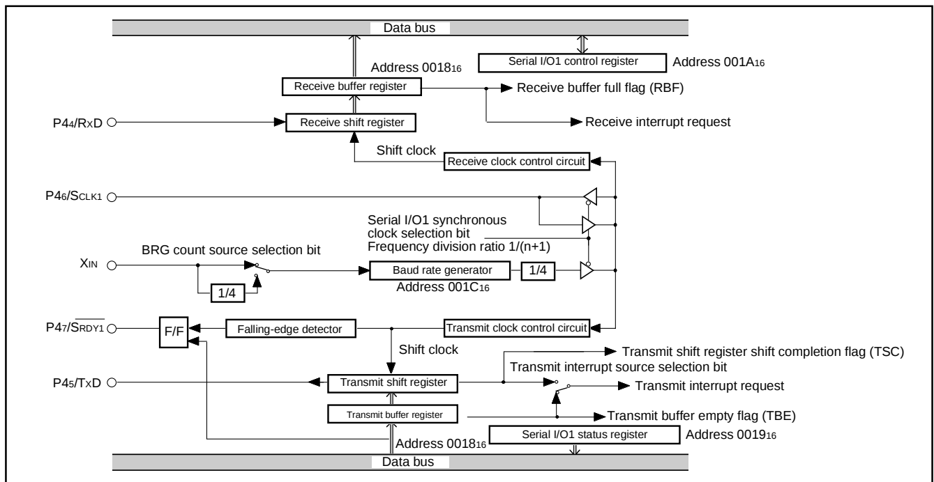
Fig. 28 Block diagram of clock synchronous serial I/O1
