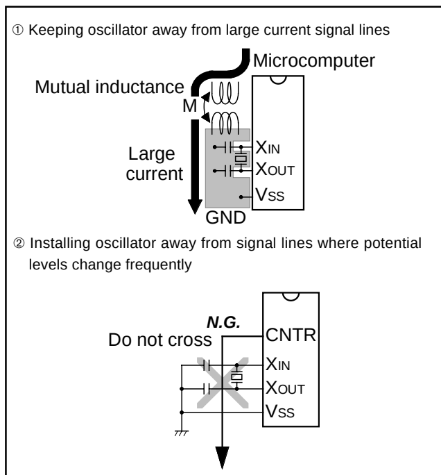
Fig. 66 Wiring for a large current signal line/Wiring of signal lines where potential levels change frequently
