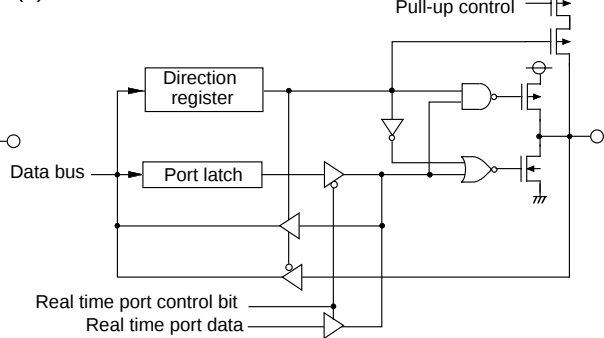
(9) Ports P52,P53
