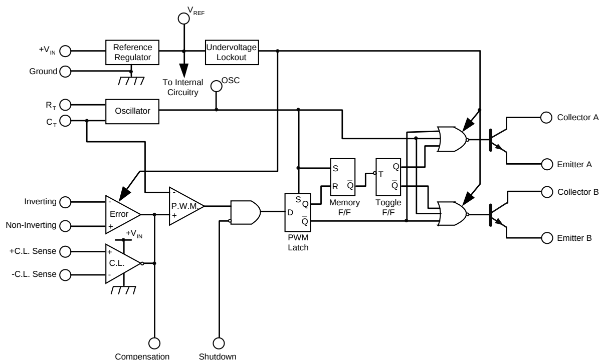
Figure 5 • Block Diagram
