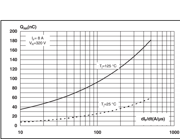
Figure 7. Reverse recovery charges versus dl_F/dt (typical values)
