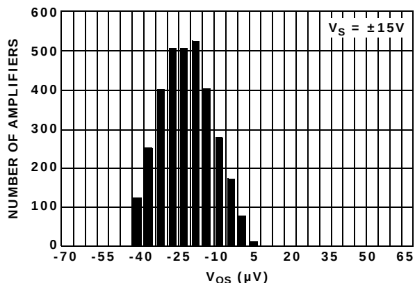
FIGURE 13. INPUT OFFSET VOLTAGE DISTRIBUTION, V_S = \pm 15V
