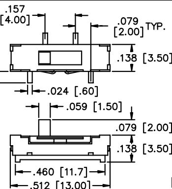
MECHANICAL OUTLINE
