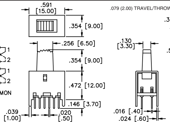
MECHANICAL OUTLINE
