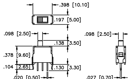
MECHANICAL OUTLINE
