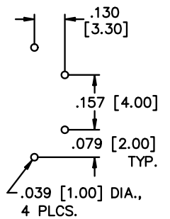
P.C. BOARD CUTOUT
