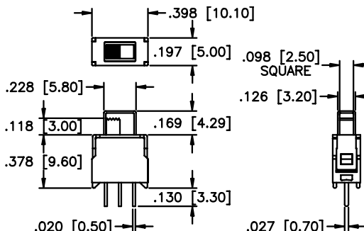
MECHANICAL OUTLINE
