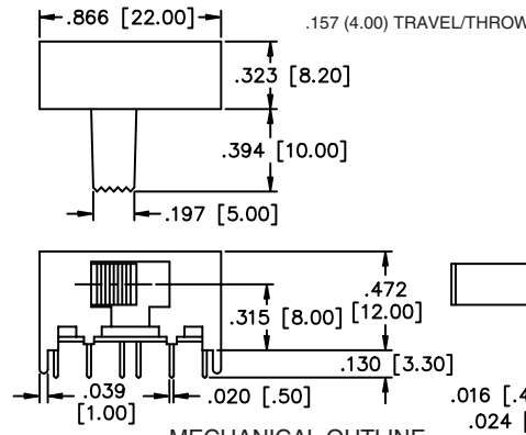
MECHANICAL OUTLINE
