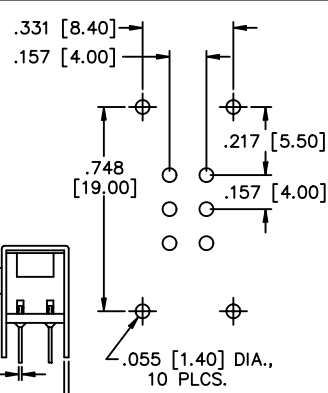
P.C. BOARD LAYOUT
