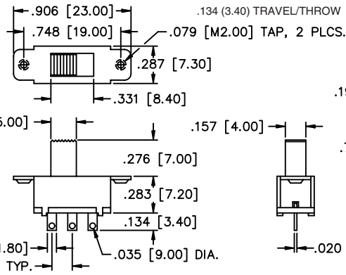
MECHANICAL OUTLINE
