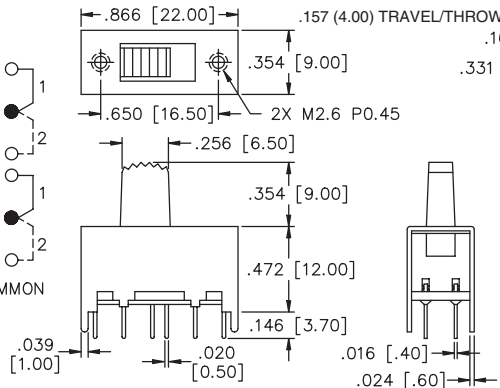
MECHANICAL OUTLINE
