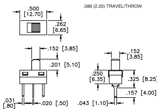
MECHANICAL OUTLINE
