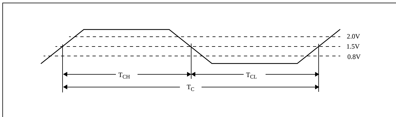
Figure 4. Clocking Waveform
