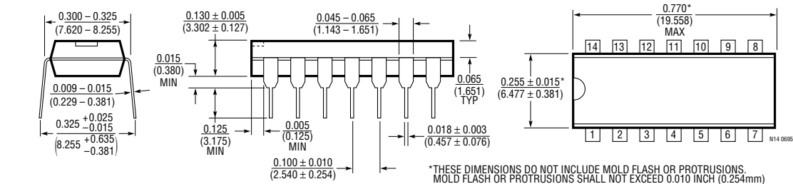
S Package 14-Lead Plastic SO
