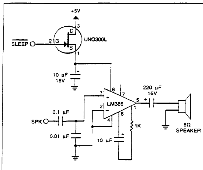
Figure 5. Speaker Control Circuit – optional to allow for call progress monitoring.
