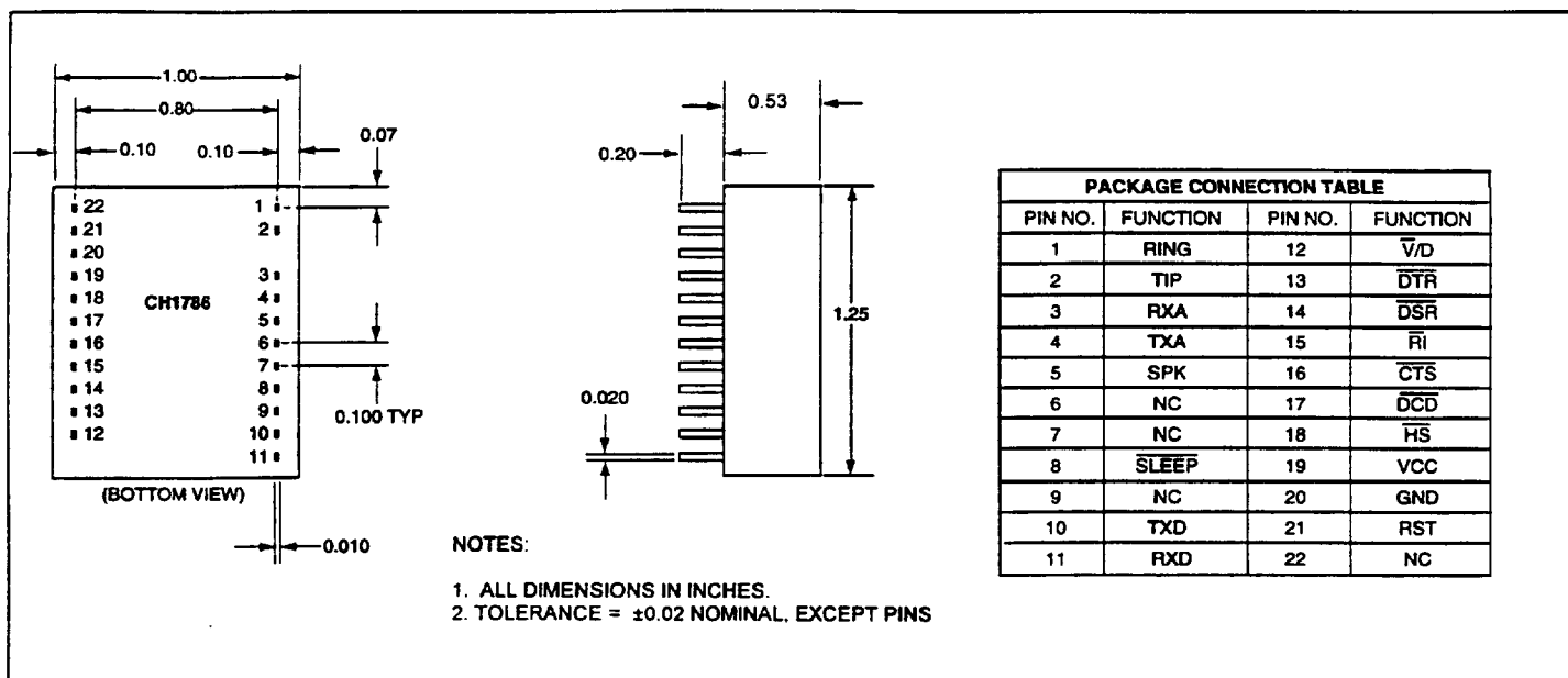
Figure 7. CH1786 Physical Dimensions and Pin Functions.
