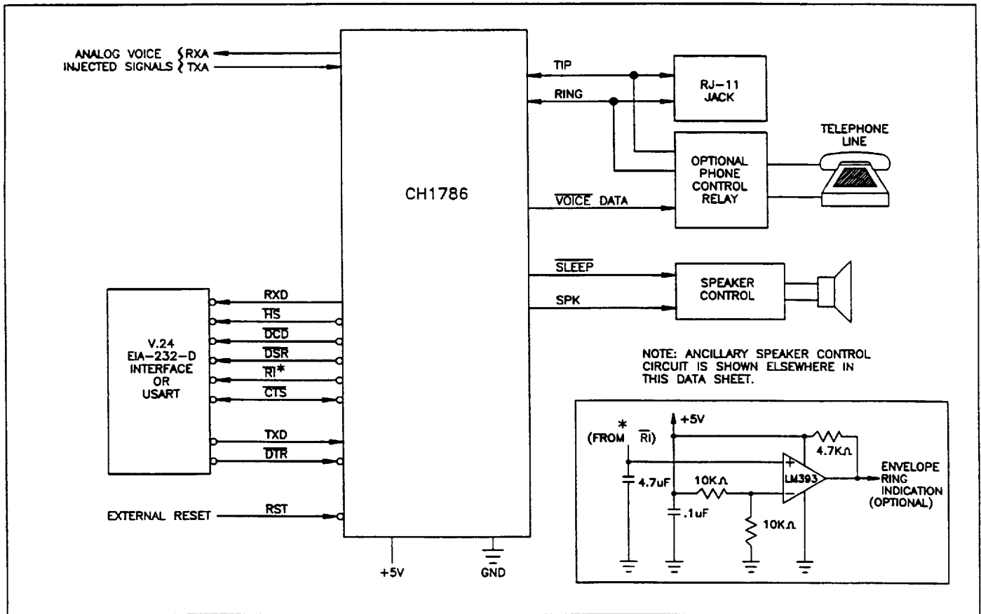
Figure 4. CH1786 Application Diagram
