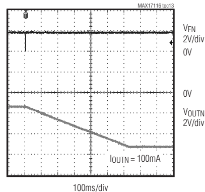
BUCK-BOOST REGULATOR TRANSITION BEHAVIOR (LATER TRANSITION FROM -1.5V TO -5.4V)
