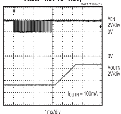
BUCK-BOOST REGULATOR TRANSITION BEHAVIOR (FIRST TRANSITION FROM -4.9V TO -1.5V)
