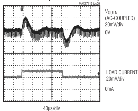
BUCK-BOOST REGULATOR LOAD TRANSIENT (20mA \leftrightarrow 30mA)
