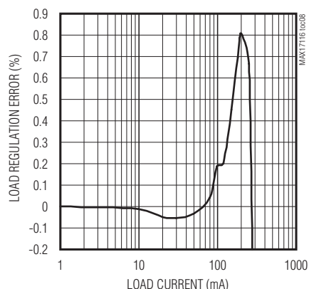
BUCK-BOOST REGULATOR OUTPUT LOAD REGULATION vs. LOAD CURRENT
