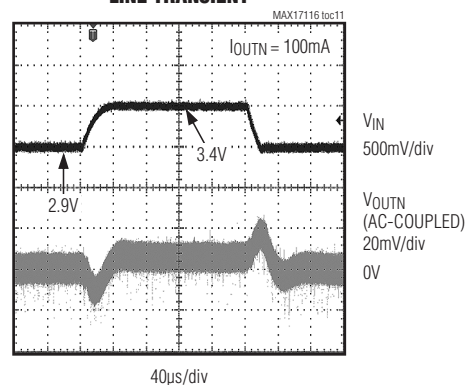
BUCK-BOOST REGULATOR LINE TRANSIENT
