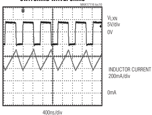
BUCK-BOOST REGULATOR SWITCHING WAVEFORMS
