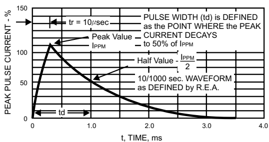
FIG.3- PULSE WAVEFORM
