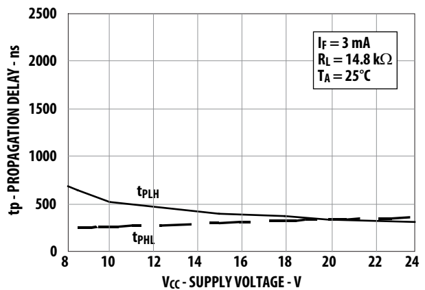
Figure 23 Typical Propagation Delay vs. Supply Voltage (ACPL-054L/W50L/K454L)
