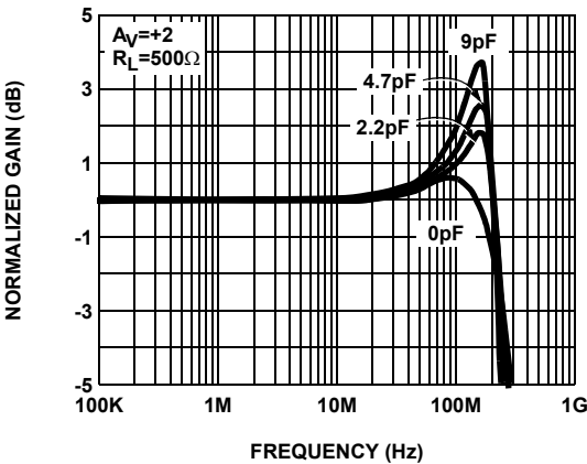
FIGURE 2. GAIN vs FREQUENCY FOR VARIOUS C_{LOAD}
