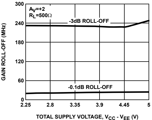
FIGURE 4. GAIN ROLL-OFF
