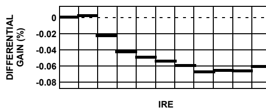
FIGURE 16. DIFFERENTIAL GAIN
