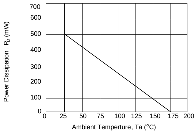
Derating Curve
