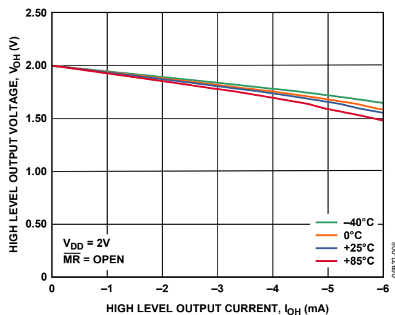
Figure 9. High Level Output Voltage vs. High Level Output Current
