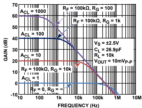
FIGURE 8. FREQUENCY RESPONSE vs CLOSED LOOP GAIN
