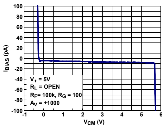
FIGURE 17. INPUT BIAS CURRENT vs COMMON-MODE INPUT VOLTAGE
