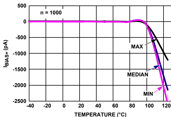
FIGURE 22. I_{BIAS+} vs TEMPERATURE V_+ = 5V , V_- = 0V
