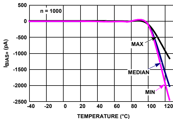
FIGURE 24. I_{BIAS+} vs TEMPERATURE V_+ = 5V , V_- = 0V
