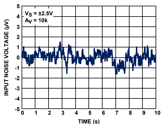
FIGURE 12. 0.1Hz TO 10Hz INPUT VOLTAGE NOISE
