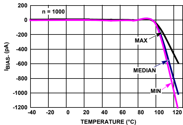
FIGURE 25. I_{BIAS-} vs TEMPERATURE V_+ = 5V , V_- = 0V
