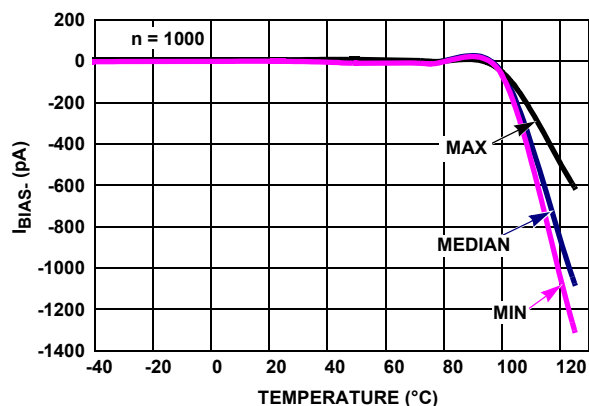
FIGURE 23. I_{BIAS-} vs TEMPERATURE V_+ = 5V , V_- = 0V
