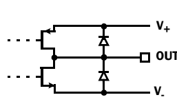
CIRCUIT 3
