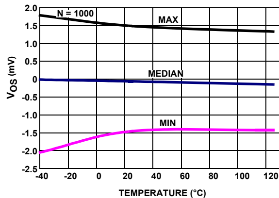
FIGURE 21. V_{OS} vs TEMPERATURE V_{IN} = 0V , V_+ = 5V , V_- = 0V
