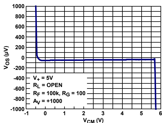
FIGURE 16. INPUT OFFSET VOLTAGE vs COMMON MODE INPUT VOLTAGE
