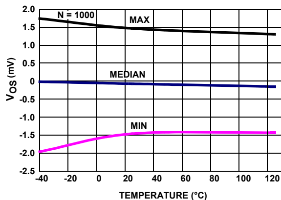
FIGURE 20. V_{OS} vs TEMPERATURE, V_{IN} = 0V , V_+ = 5V , V_- = 0V
