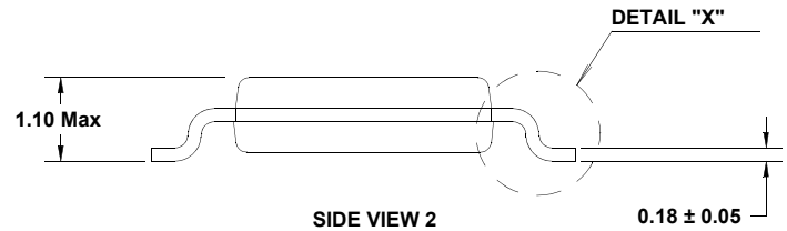
SIDE VIEW 2
