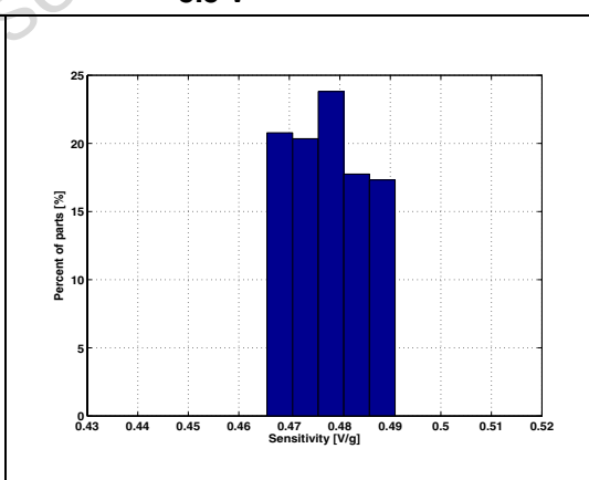
Figure 8. Y axis sensitivity-g level at 3.3 V
