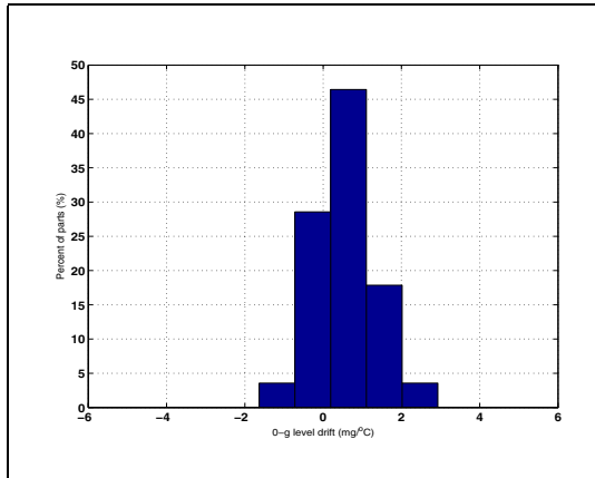
Figure 13. Y axis zero-g level change vs. temperature at 3.3 V
