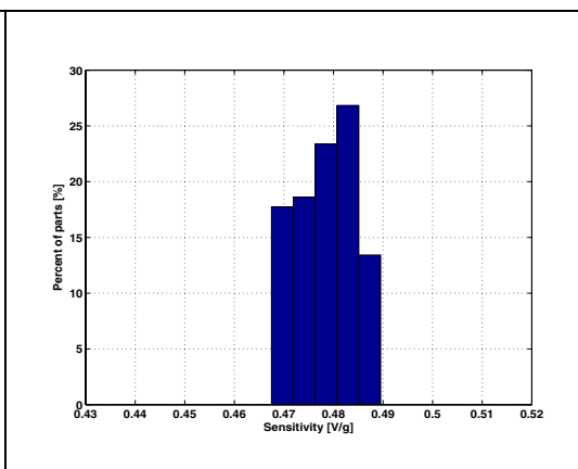
Figure 10. Z axis sensitivity-g level at 3.3 V
