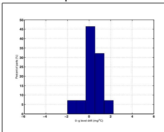
Figure 15. Z axis zero-g level change vs. temperature at 3.3 V
