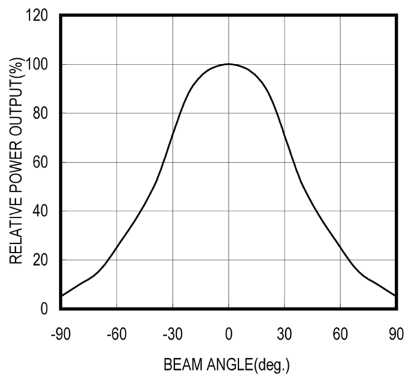
RADIATION PATTERN
