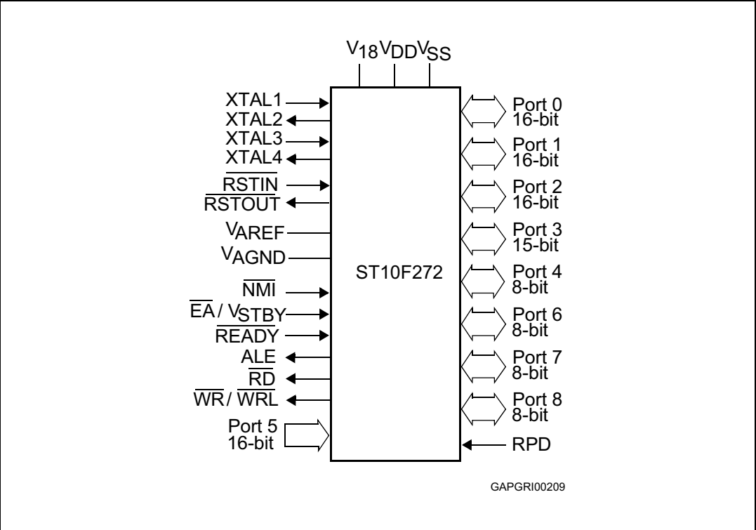
Figure 1. Logic symbol
