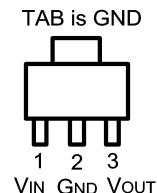
Figure 2. SOT-223 Top View See Package Number DCY0004A
