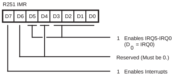
Figure 33. Interrupt Mask Register (FB H : Read/Write)
