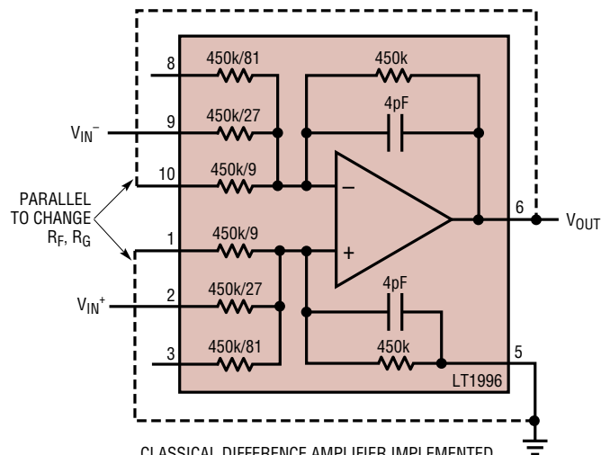
CLASSICAL DIFFERENCE AMPLIFIER IMPLEMENTED WITH LT1996. R F = 450k, R G = 16.7k, GAIN = 3.
