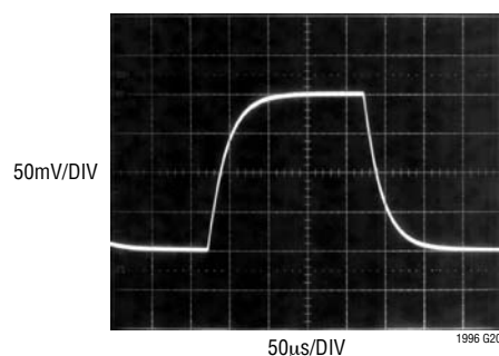
Small Signal Transient Response, Gain = 81
