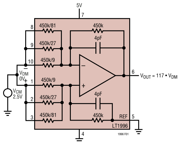
Figure 1. Difference Amplifier Cannot Produce 0V on a Single Supply. Provide a Negative Supply, or Raise Pin 5, or Provide 400μV of V_{DM}
