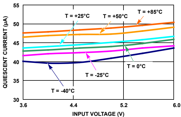
FIGURE 6. QUIESCENT CURRENT vs INPUT VOLTAGE ( V_{OUT2} = 3.3V , ONLY LD02 ENABLED)
