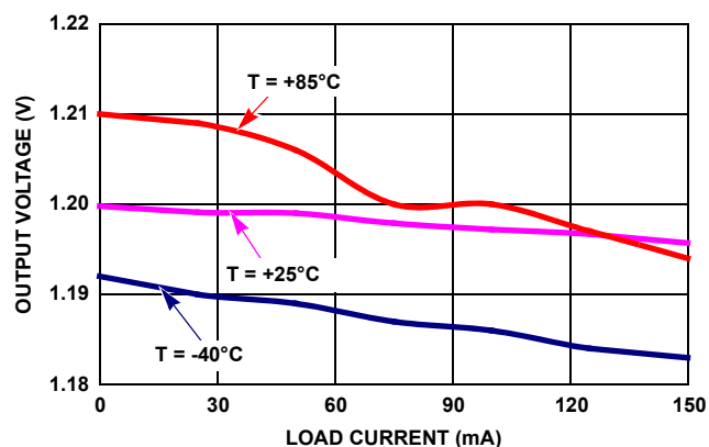
FIGURE 10. LOAD REGULATION ( V_{IN} = 1.8V , V_{OUT} = 1.2V )
