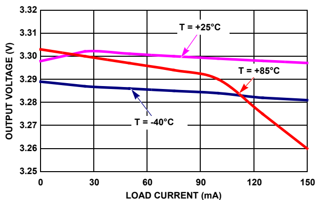
FIGURE 11. LOAD REGULATION ( V_{IN} = 4.5V , V_{OUT} = 3.3V )
