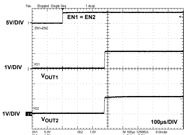
FIGURE 12. ENABLE OPERATION ( V_{IN} = 3.6V , V_{OUT1} = V_{OUT2} = 1.2V )
