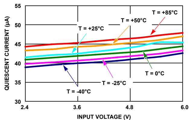
FIGURE 3. QUIESCENT CURRENT vs INPUT VOLTAGE ( V_{OUT2} = 2.1V , ONLY LD02 ENABLED)
