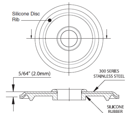
Bottom View- Facing Contact Surface
