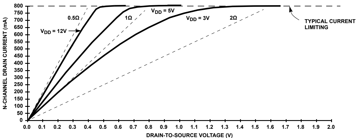
FIGURE 7. TYPICAL CHARACTERISTIC OF THE N-MOSFET OUTPUT DRIVER DRAIN CURRENT vs DRAIN-TO-SOURCE VOLTAGE, T_{\text{AMBIENT}} = 25^{\circ}\text{C}
