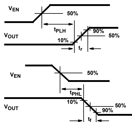
FIGURE 3. SWITCHING WAVEFORMS
