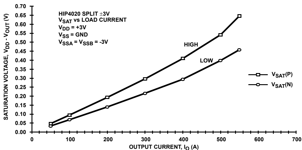
FIGURE 10. TYPICAL CHARACTERISTIC OF SATURATION VOLTAGE vs OUTPUT CURRENT USING A \pm 3V SPLIT SUPPLY, OUTPUT REFERENCE EQUAL LOGIC GROUND, T_{AMBIENT} = 25^{\circ}C
