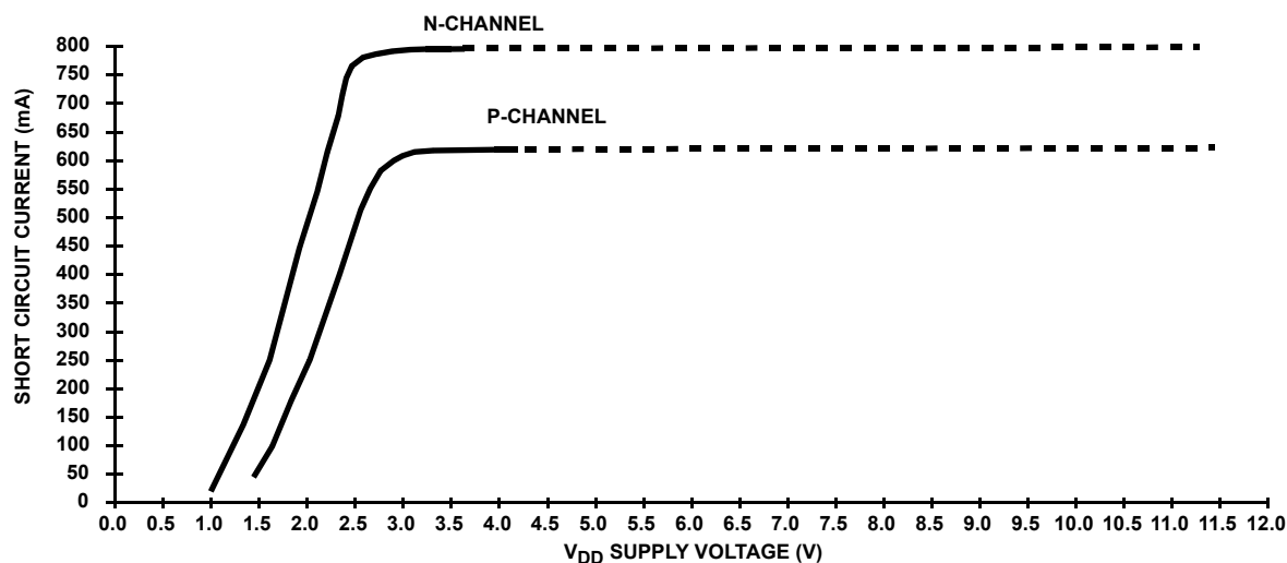
FIGURE 8. TYPICAL CHARACTERISTIC OF THE P AND N OUTPUT DRIVER SHORT CIRCUIT CURRENT vs SUPPLY VOLTAGE, T_{\text{AMBIENT}} = 25^{\circ}\text{C}
