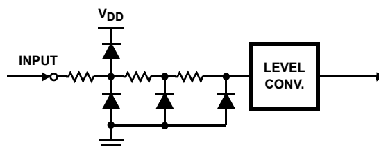
FIGURE 4. LOGIC INPUT ESD INTERFACE PROTECTION
