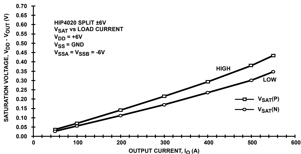
FIGURE 11. TYPICAL CHARACTERISTIC OF SATURATION VOLTAGE vs OUTPUT CURRENT USING A \pm 6V SPLIT SUPPLY, OUTPUT REFERENCE EQUAL LOGIC GROUND, T_{AMBIENT} = 25^{\circ}C
