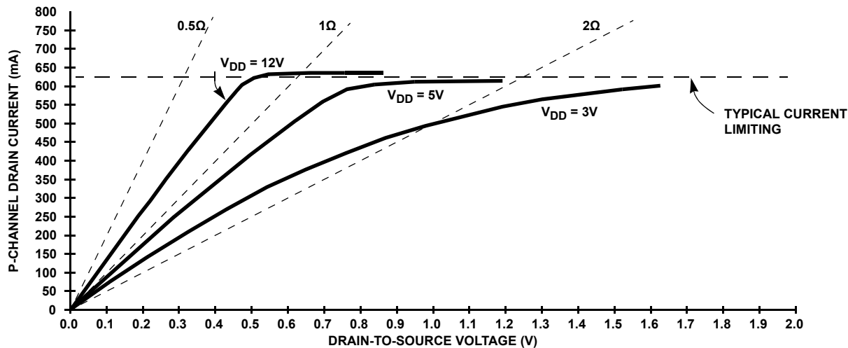
FIGURE 6. TYPICAL CHARACTERISTIC OF THE P-MOSFET OUTPUT DRIVER DRAIN CURRENT vs DRAIN-TO-SOURCE VOLTAGE, T_{\text{AMBIENT}} = 25^{\circ}\text{C}
