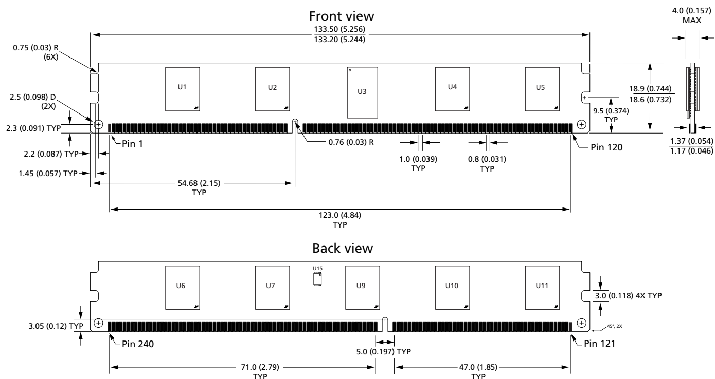
Figure 3: 240-Pin DDR3 RDIMM
