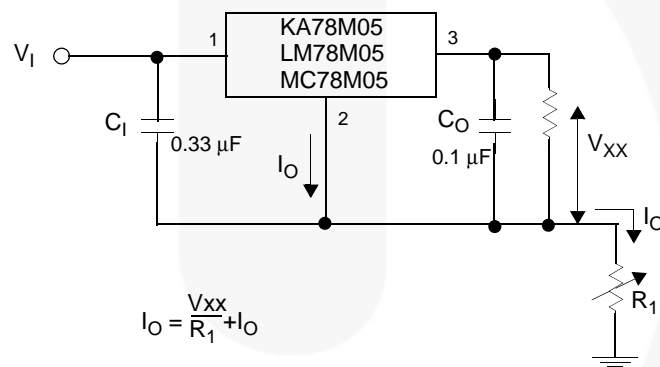
Figure 3. Constant-Current Regulator
