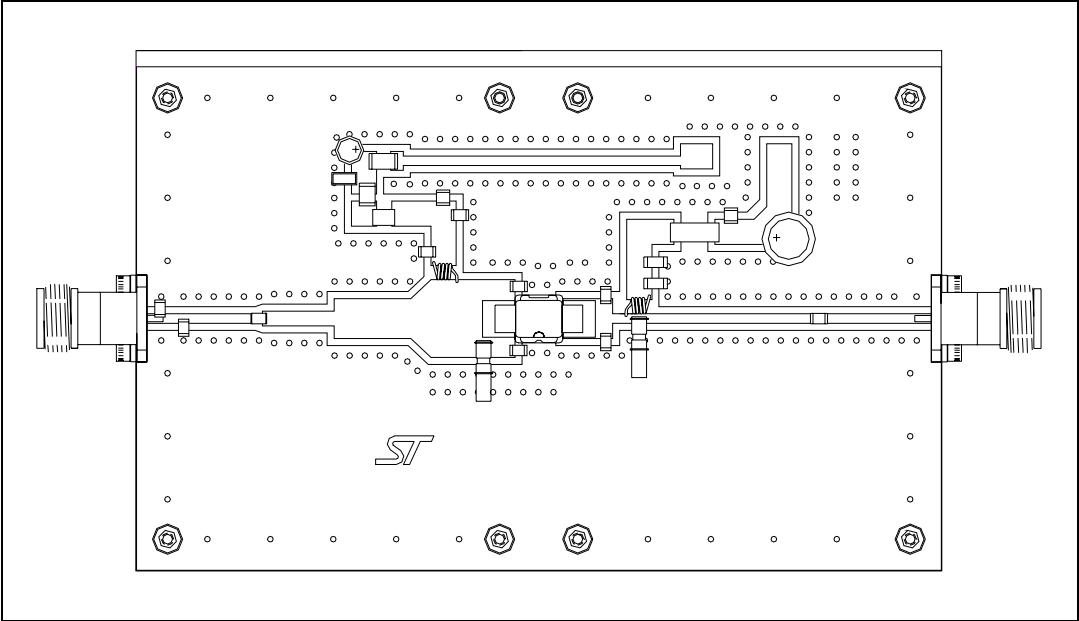
Figure 16. Test circuit
