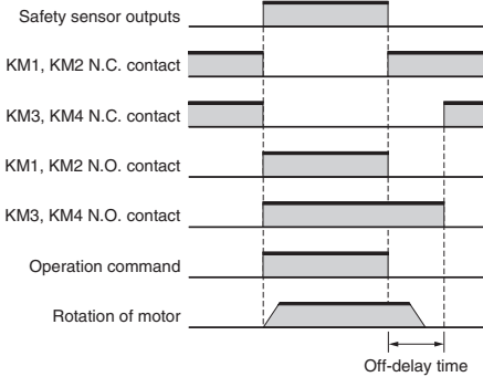
Timing chart
