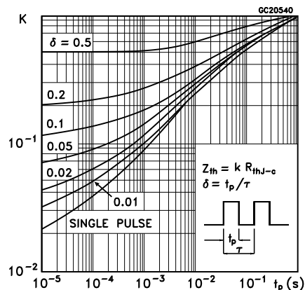
Figure 2. Thermal impedance
