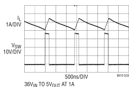
Switching Waveforms
