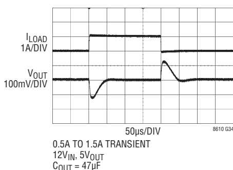
Transient Response
