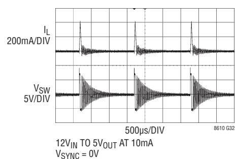
Switching Waveforms
