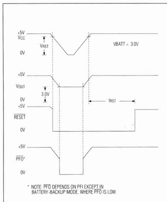
Figure 2. Timing Diagram
