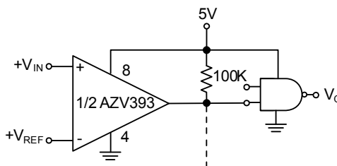
Driving CMOS
