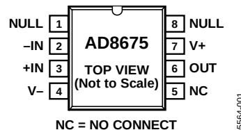
Figure 1. 8-Lead SOIC_N (R-8)
