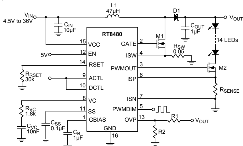
Figure 3. True PWM Dimming in Boost Configuration
