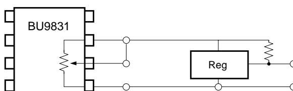
Fig.21 Variable output adjustment of regulator
