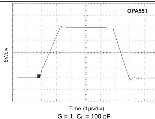
Figure 20. Large-Signal Step Response OPA551
